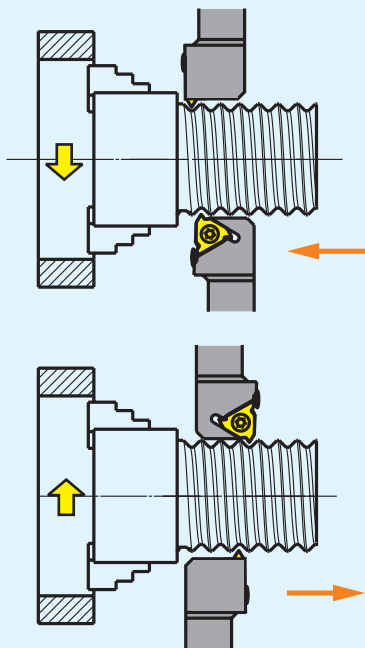
External threading machining (Right thread)
